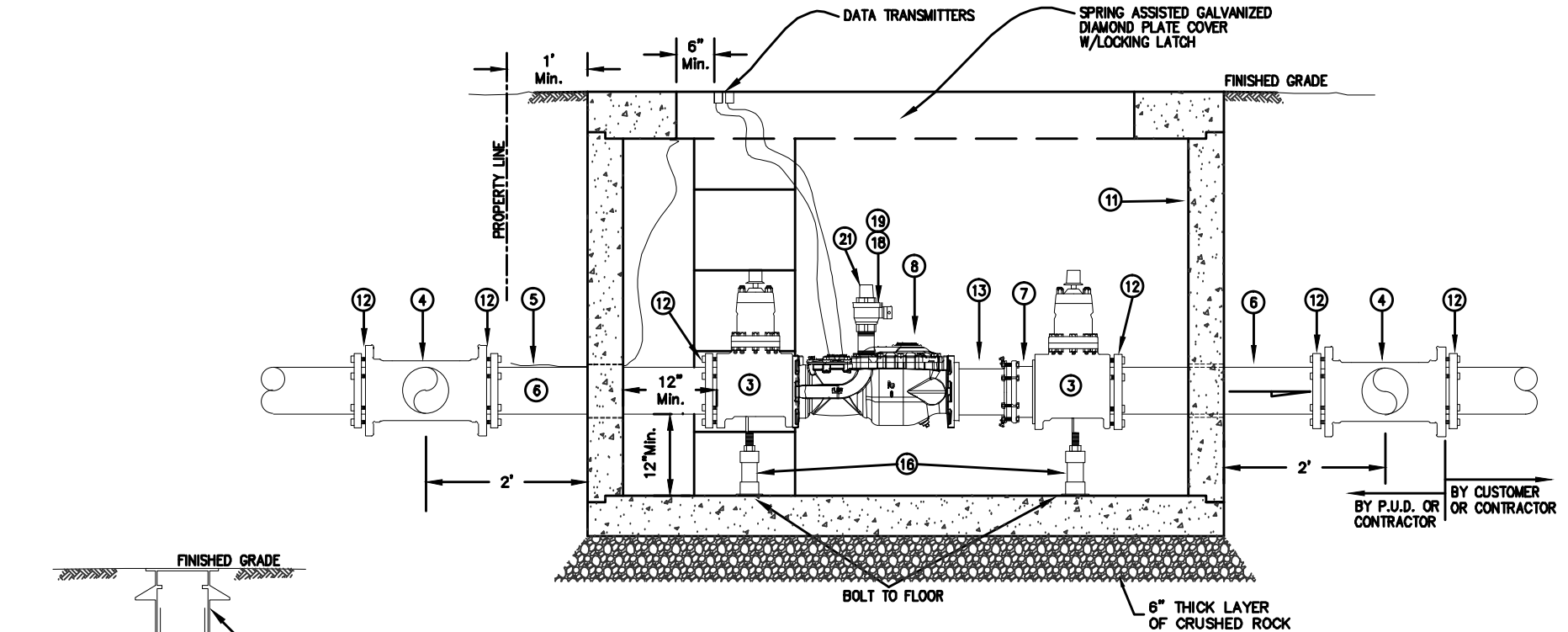
ELEVATION REFER TO SHEET 1/2 FOR PLAN VIEW
