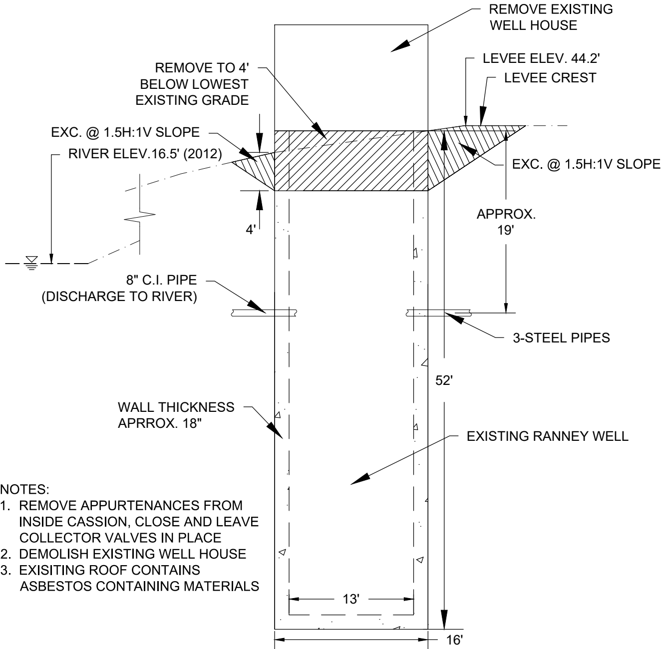
RANNEY WELL CASSION (SCHEMATIC) N.T.S.
